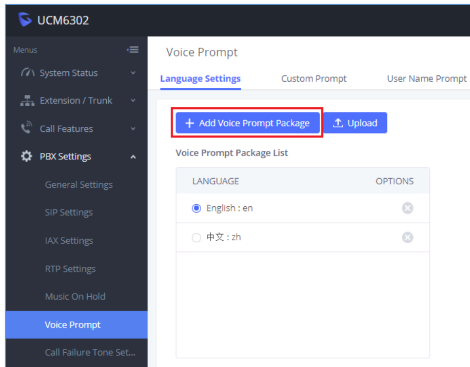
Figure 149: Language Settings for Voice Prompt
