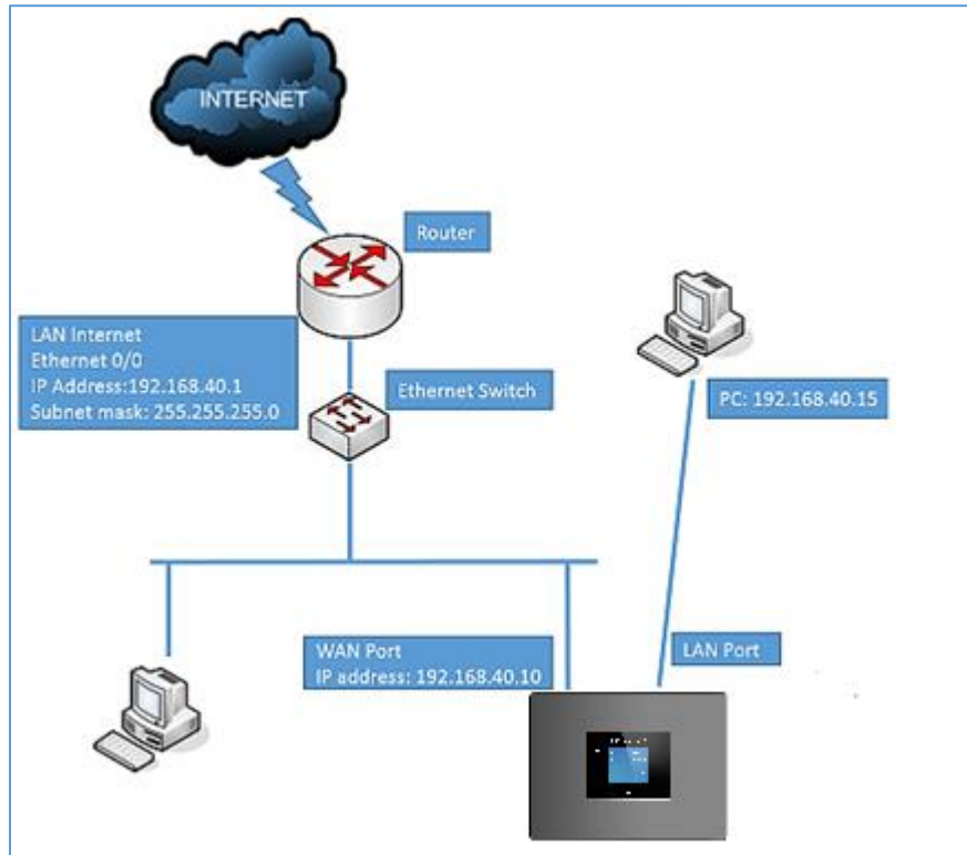
Figure 16: UCM6302 Network Interface Method: Switch
