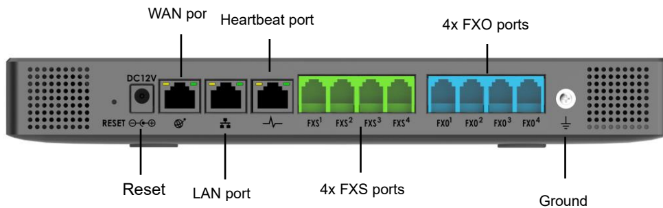
Figure 6: UCM6304 Back View
