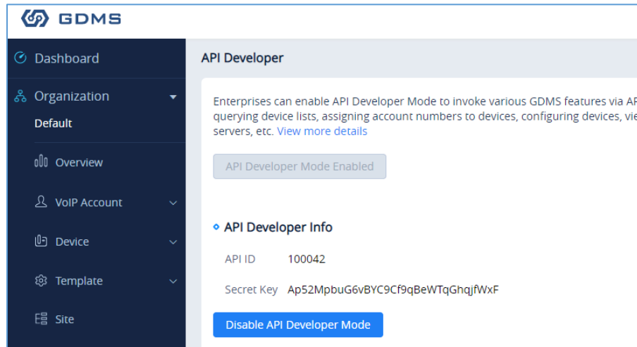
Figure 54: GDMS API Credentials
