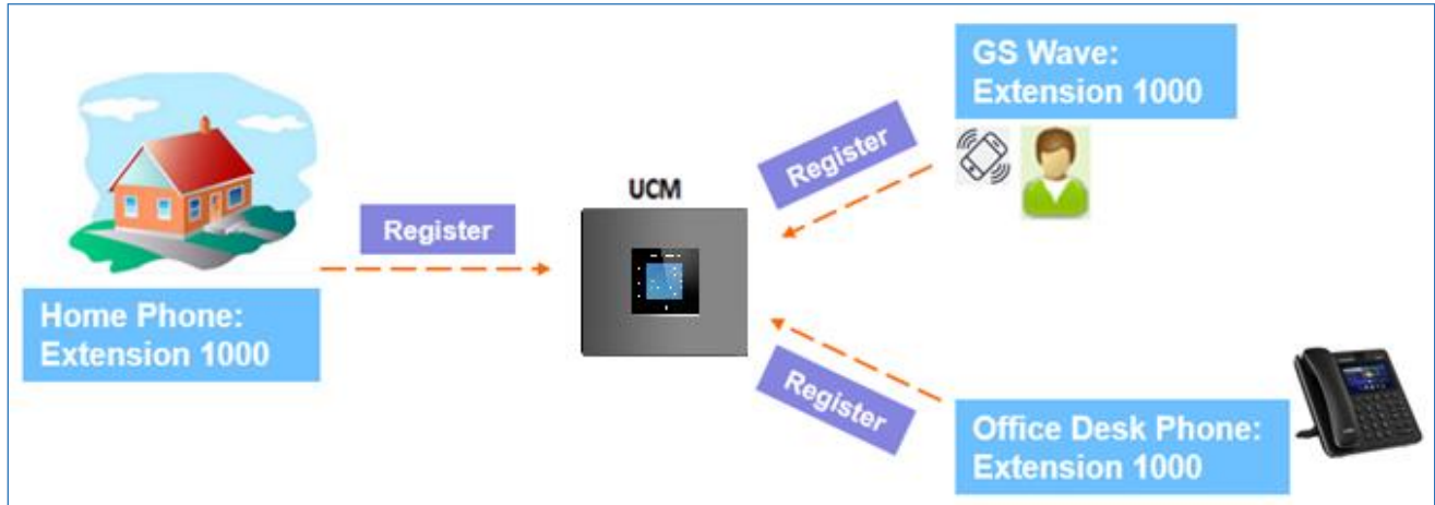
Figure 92: Multiple Registrations per Extension
