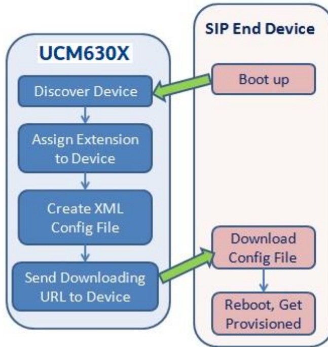
Figure 59: UCM630X Zero Config
