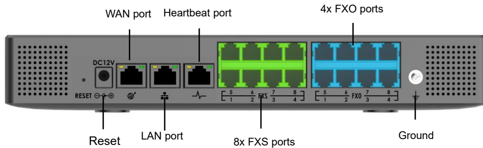
Figure 8: UCM6308 Back View
