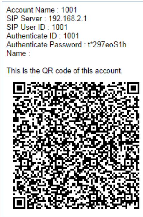
Figure 90: Account Registration Information and QR Code
