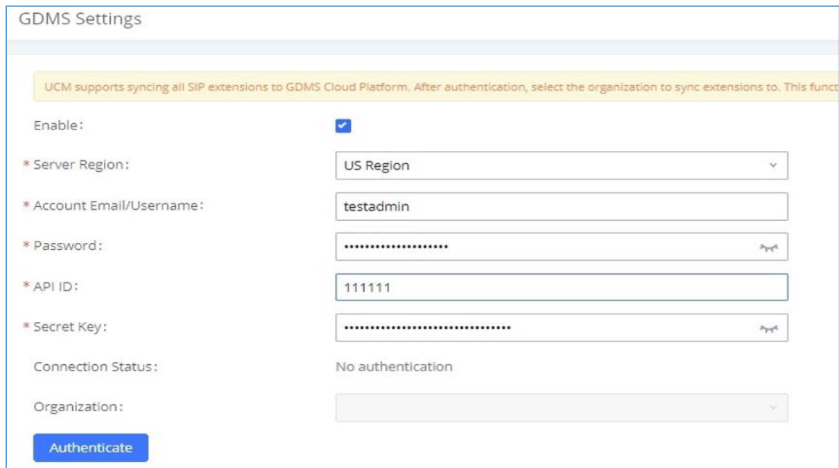
Figure 55: GDMS configuration on the UCM
